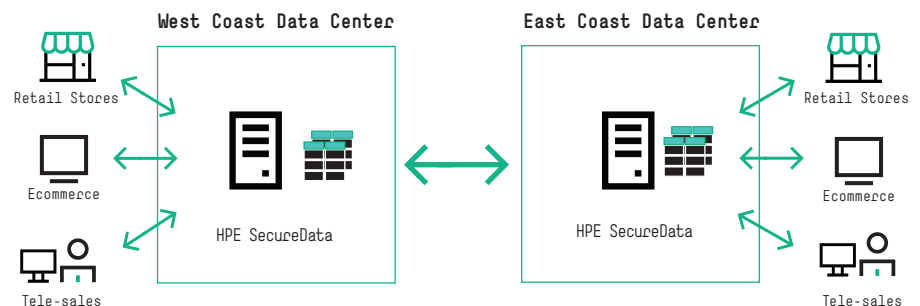
Figure 2. HPE SecureData tokenization: one-time distribution of static token tables
