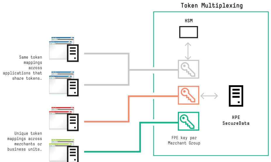
Figure 3. HPE SecureData Token Multiplexing simplifies token independence between merchants, applications, and line of business, avoiding the hassle using multiple databases
