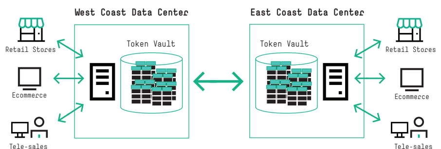
Figure 1. Ideal data path for traditional protection approach.
