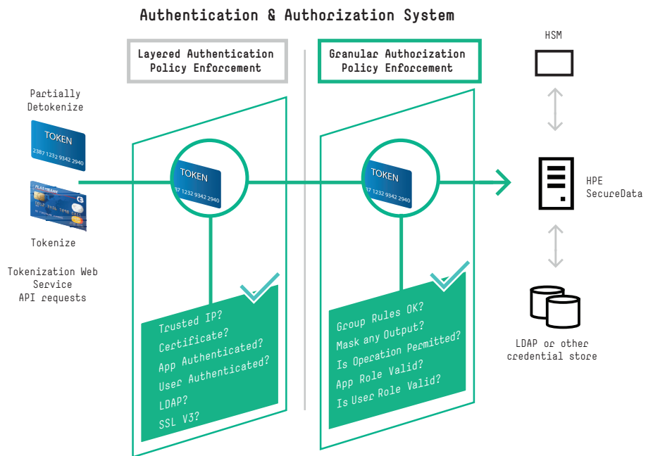
Figure 4. HPE SecureData supports tokenization best practices, authenticating both users and applications
